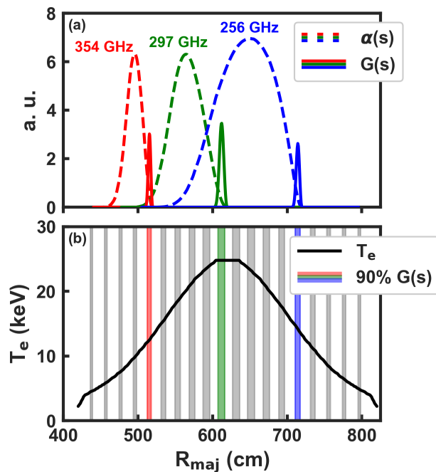
FIG. 4: (a) The absorption coefficients \alpha(s) and emissivity functions G(s) are plotted as functions of major radius R_{maj} for three selected second harmonic ECE frequencies on ITER. (b) The temperature profile T_e(R_{maj}) assumed for these calculations is an H-mode discharge with T_{e,max} = 25 keV. The 90% width of each ECE frequency is over-plotted as vertical bars, showing measurement limitations due to broadening.
