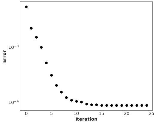
FIG. 7: The error of the PSIRZ/ T_e symmetry and q(R) as a function of iteration number.
