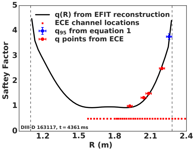
FIG. 2: Comparison between (black curve) equilibrium reconstruction from external magnetics and E_R -corrected MSE constraints 31 and (red points) the radial locations of the m/n = 1/1, 5/2, 4/3 and 6/4 modes found with ECE for DIII-D discharge 163117 at t = 4361 ms. Four modes can be found within the available ECE coverage. Also shown is an approximation for q_{95} from equation 1 (blue point.)
