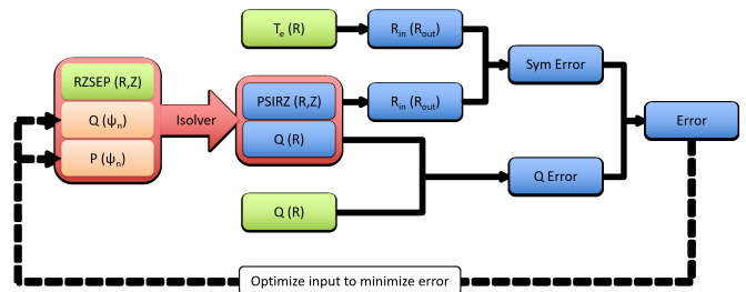
FIG. 5: Schematic of the equilibrium-selection process using ECE and Isolver. Green boxes represent measured quantities, blue boxes represent calculated quantities, and orange boxes represent guessed profiles fed to Isolver. A 'best fit' equilibrium is chosen by minimizing the error between the the measured and calculated q(R) profiles and the symmetry mappings R_{out}(R_{in}) of the calculated poloidal flux and the measured electron temperature.
