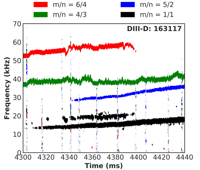
FIG. 1: Spectrogram of the Mirnov signal for DIII-D discharge 163117, showing m/n = 1/1, 5/2, 4/3 and 6/4 modes at t = 4361 ms.
