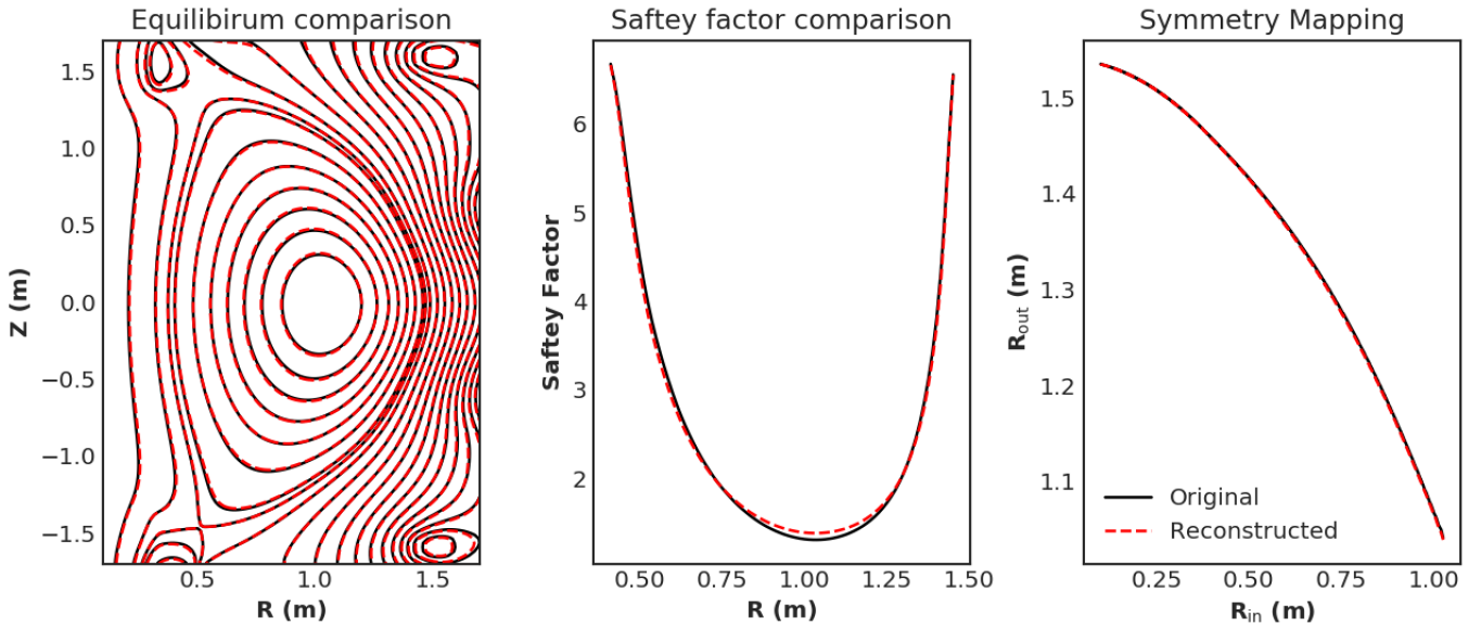
FIG. 6: Comparison of equilibria generated with Isolver. The original equilibrium is plotted in black (solid) and was chosen as a random possible equilibrium for NSTX. The reconstructed equilibrium is plotted in red (dashed), and was produced by selecting a 'best fit' equilibrium using the methods described in the text.
